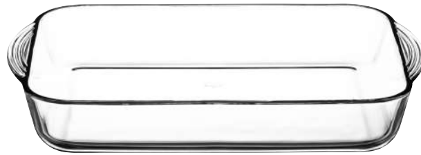
RECTANGULAR TRAY DİKDÖRTGEN TEPŞİ 59124 ~3850 cc. 128 1/4 US oz. - 135 2/4 UK oz. 60 mm. 2 1/4" 400 x 250 mm. 15 3/4 x 9 3/4" 1043141 • gb1-4ob/hk1-4dk
